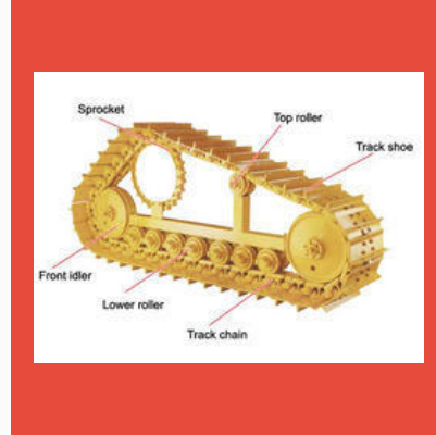
Parts of A Excavator
