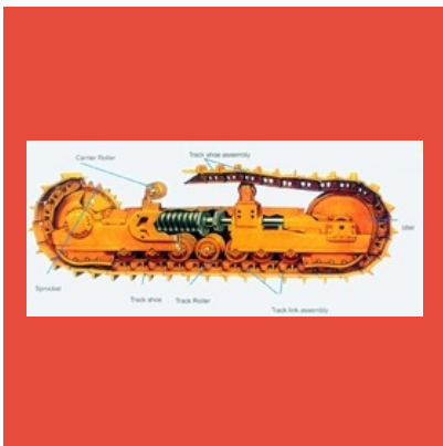
Undercarriage Parts
